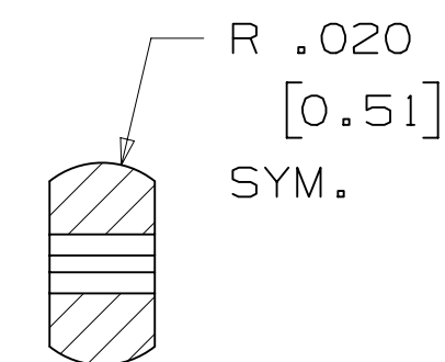
SECTION S-S
