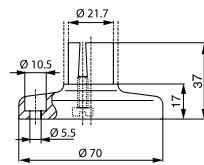
Base for Tube, Plastic
