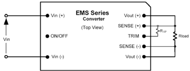
Figure 22. EMS Trim Schematic
