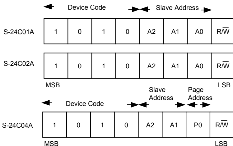
Figure 9 Device Address
