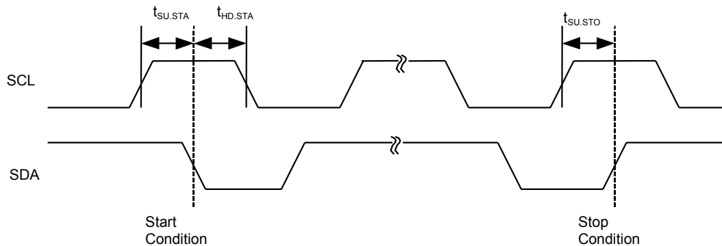
Figure 6 Start/Stop Conditions
