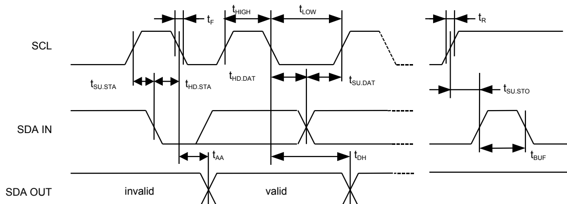
Figure 4 Bus Timing
