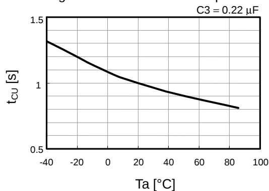
Overcurrent1 detection time vs. temperature
