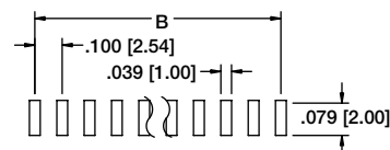
PH1RB-10-UA-SMT
