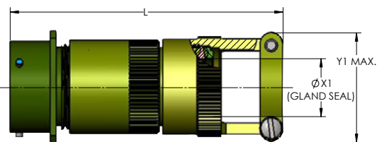
RECEPTACLE WHEN ASSEMBLED WITH BACKSHELL CLASS "J"
