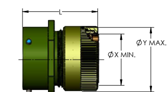
RECEPTACLE WHEN ASSEMBLED WITH BACKSHELL CLASS "E"
