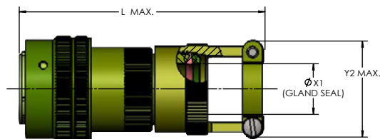
PLUG WHEN ASSEMBLED WITH BACKSHELL CLASS "J"
