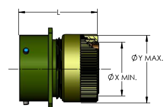
RECEPTACLE WHEN ASSEMBLED WITH BACKSHELL CLASS "E"
