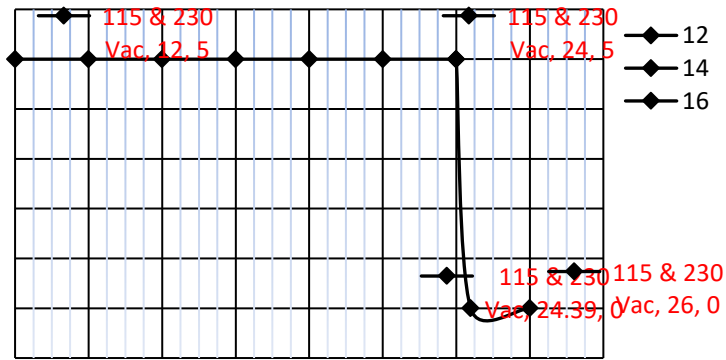
(A) Constant Current Vs Constant Voltage
