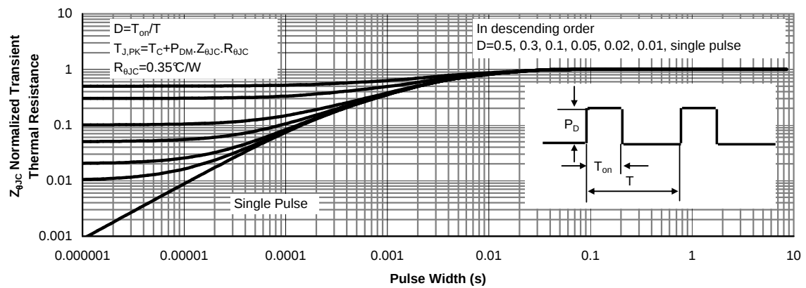
Figure 14: Normalized Maximum Transient Thermal Impedance for AOK27S60 (Note F)
