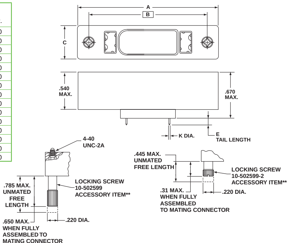
Input/Output Connector
