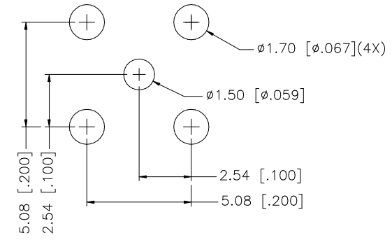
PCB MOUNTING HOLES
