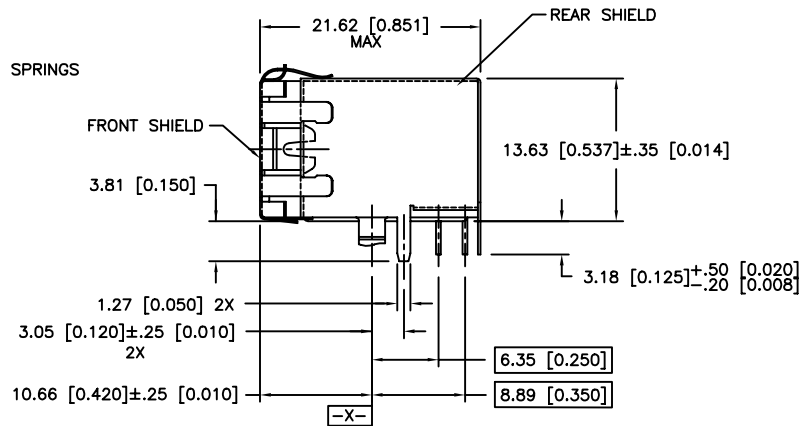
VIEW FOR 1 PORT ONLY (WITH END TABS) P/N -X010LF (SEE TABLE) DIMENSIONS SHOWN APPLY TO -X011LF PRODUCT ALSO
