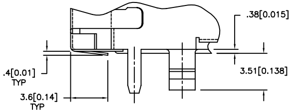
VIEW D SCALE: 2/1 DIMENSIONS ALSO APPLY TO -X010LF & -X011LF PRODUCT
