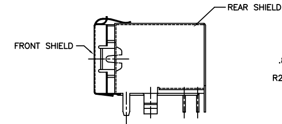
VIEW FOR 2 THRU 12 PORT (WITHOUT END TABS) P/N -XY11LF (SEE TABLE)
