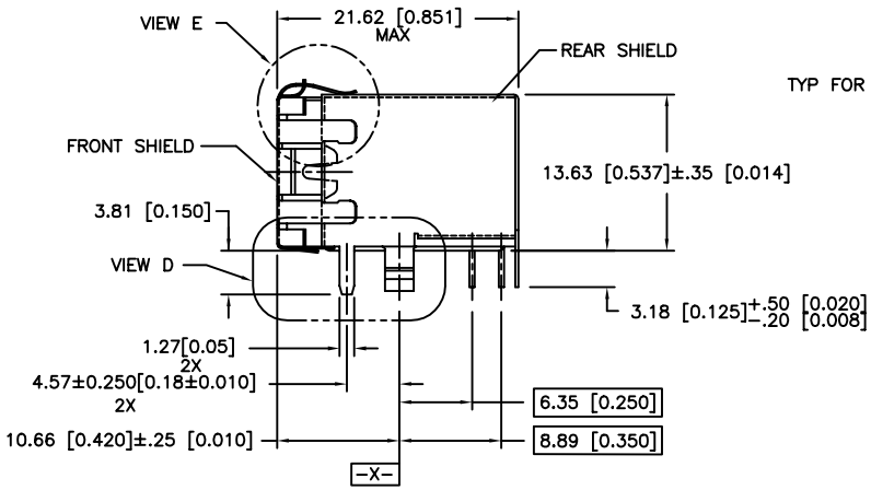
VIEW FOR 2 THRU 12 PORT (WITH END TABS) P/N -XY10LF (SEE TABLE) DIMENSIONS SHOWN APPLY TO -XY11LF PRODUCT ALSO
