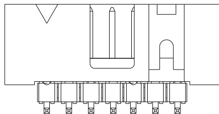
7 POSITION 2 X 7 STYLE C
