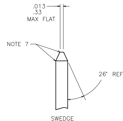
DETAIL D SCALE: 10/1 TYP BOTH ENDS
