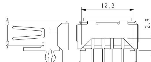
STYLE 3 WITH PARTIAL BACK SHELL
