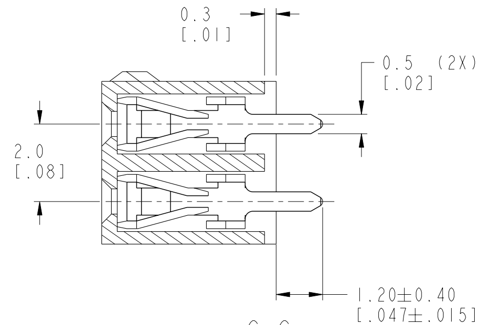
SECTION C-C
