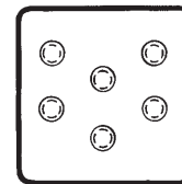
Insert 6T6 (6) Size 8 Twinax Contacts Grounded
