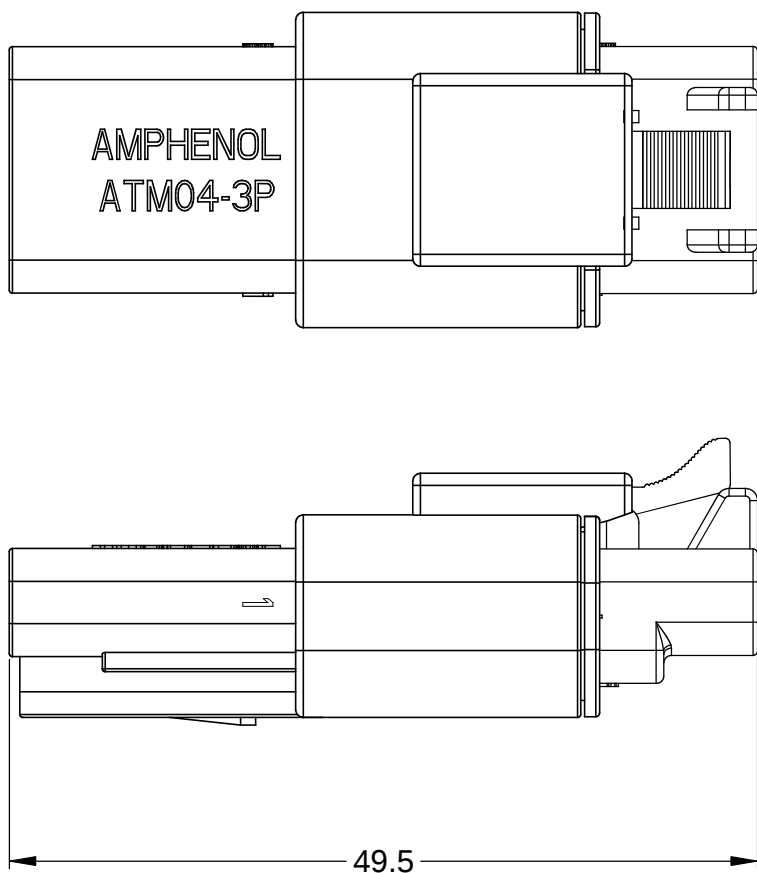
ASSEMBLED PLUG AND RECEPTACLE
