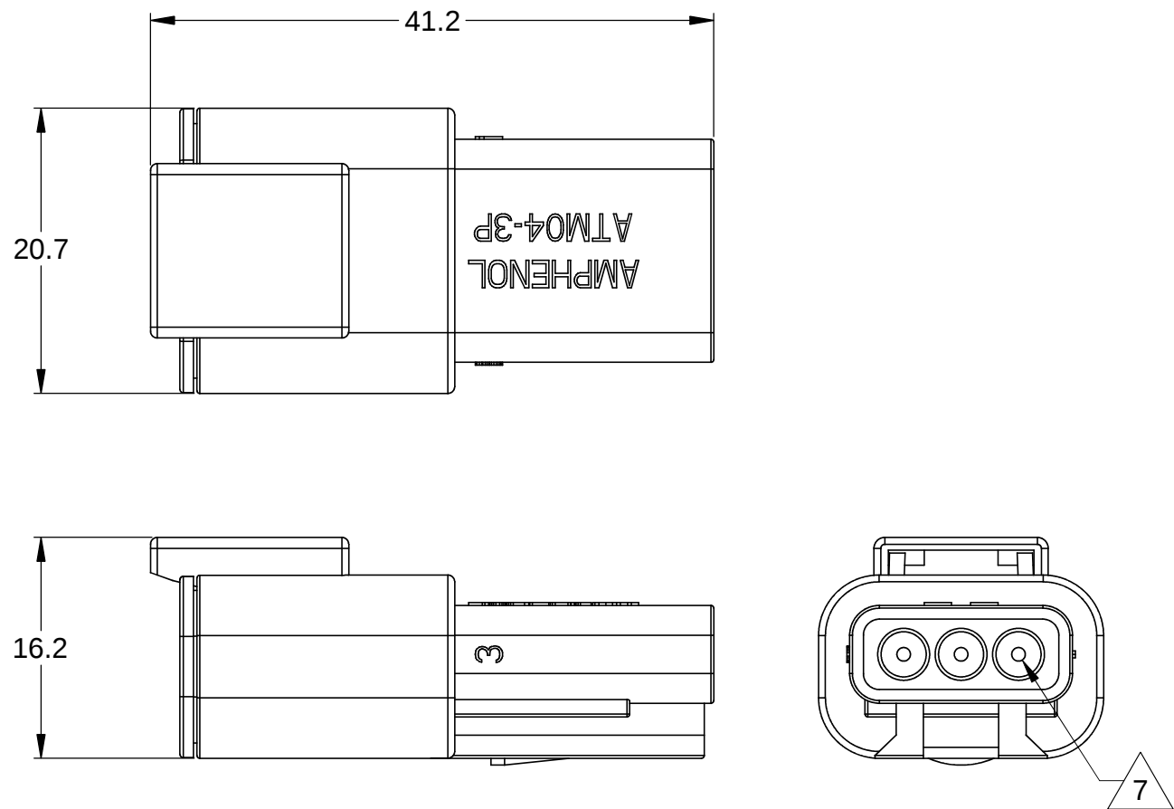
REFERENCE DIMENSIONS - ASSEMBLED RECEPTACLE
