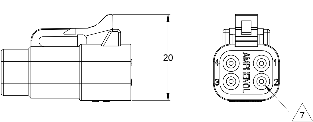
REFERENCE DIMENSIONS - ASSEMBLED PLUG
