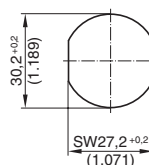
Panel cutout
