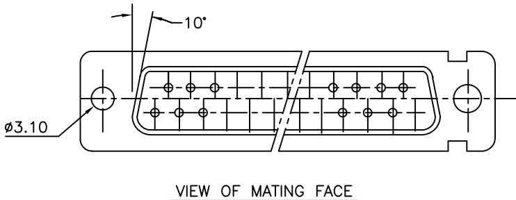
VIEW OF MATING FACE
