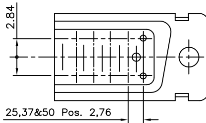
LAY OUT OF 50P CONNECTOR
