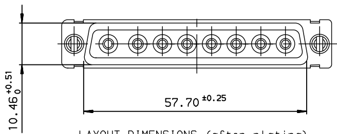
LAYOUT DIMENSIONS (after plating) CONNECTOR SIDE VIEW
