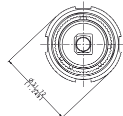
Panel Drilling
