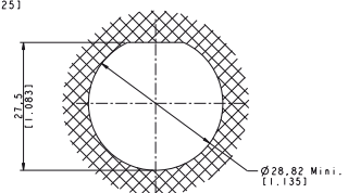
Panel Drilling
