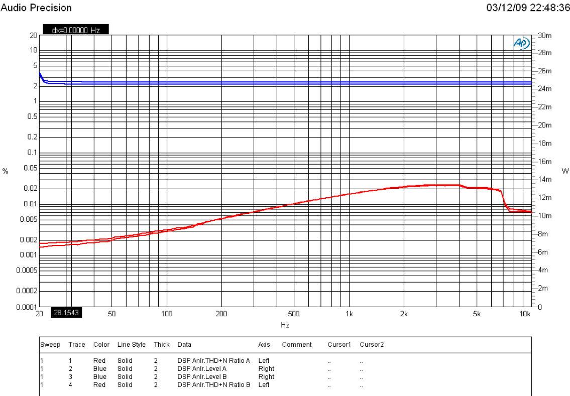
Figure 10. Typical Performance Data, FF configuration
