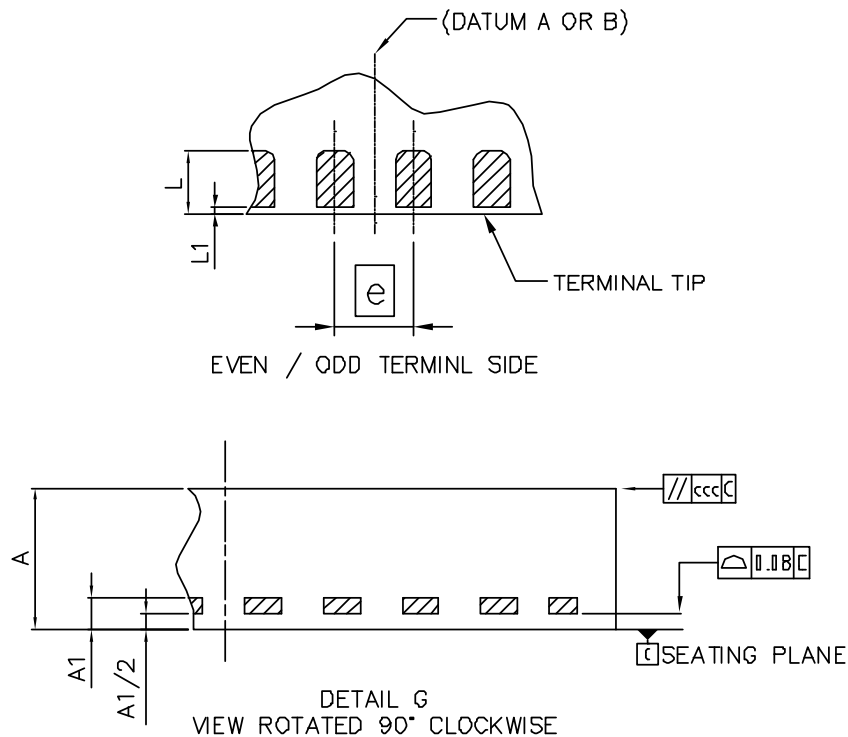
Figure 35. AS3502; QFN32 0.5mm pitch details
