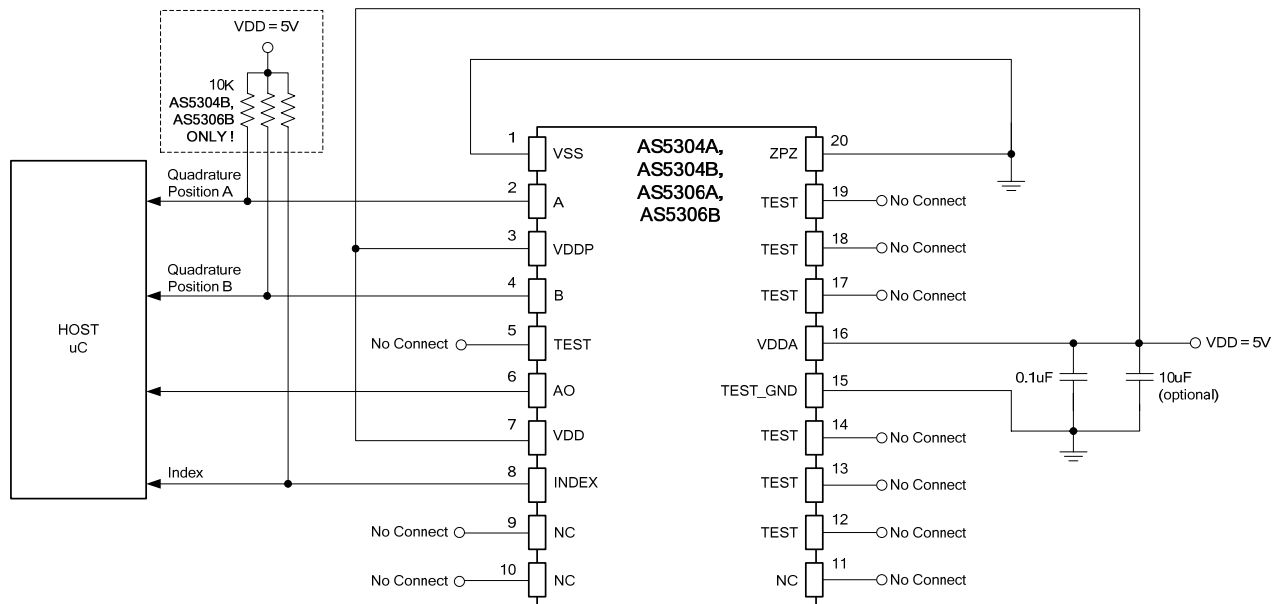
Figure 5: Electrical connection of the AS5304/AS5306
