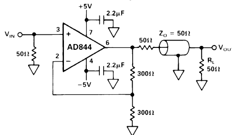
Figure 35a. The AD844 as a Cable Driver
