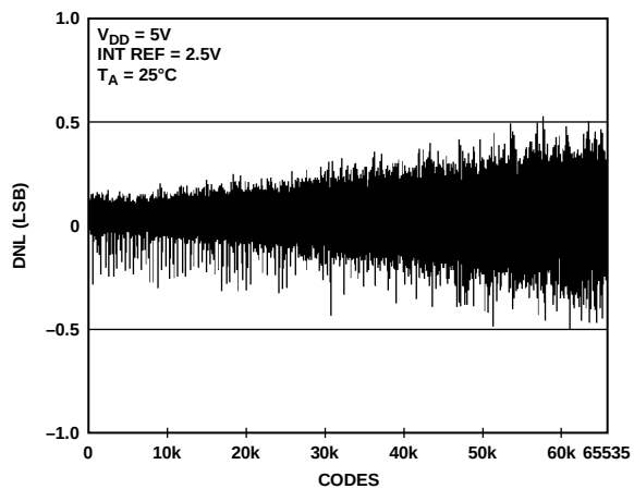
Figure 16. DNL AD5668-2/AD5668-3
