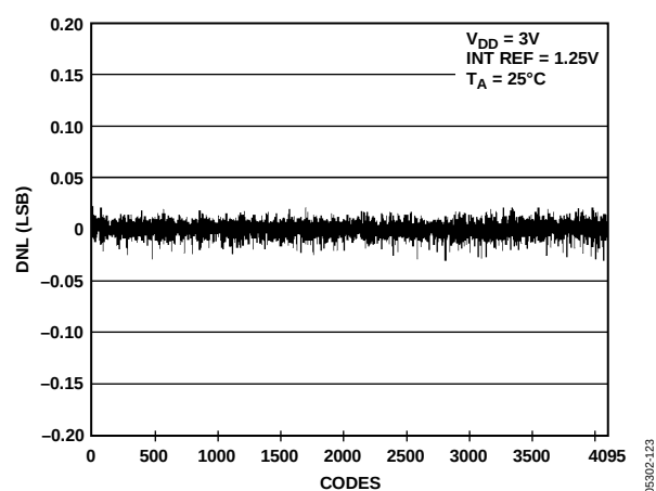
Figure 24. DNL AD5628-1
