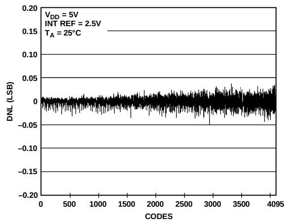
Figure 18. DNL AD5628-2
