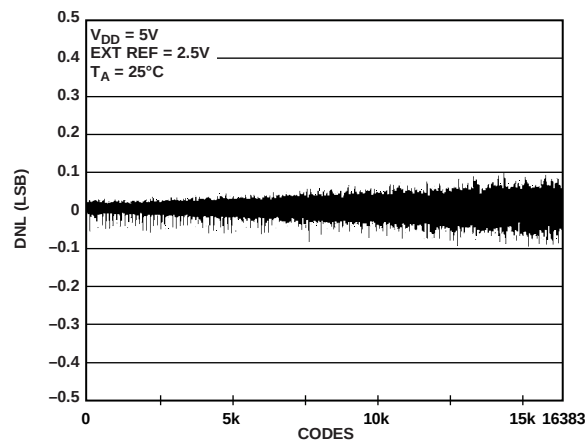
Figure 17. DNL AD5648-2
