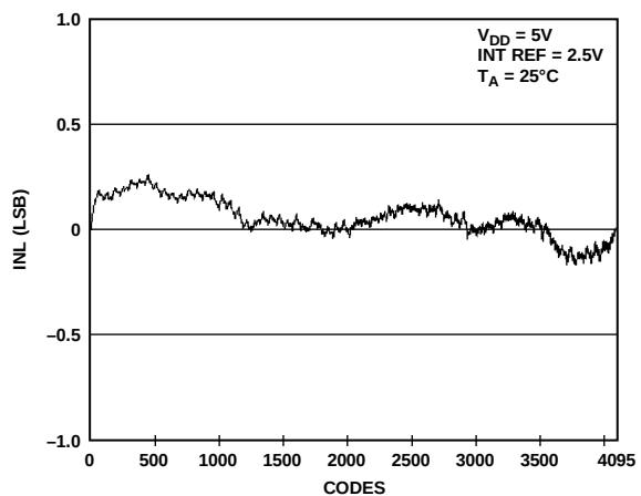
Figure 15. INL AD5628-2
