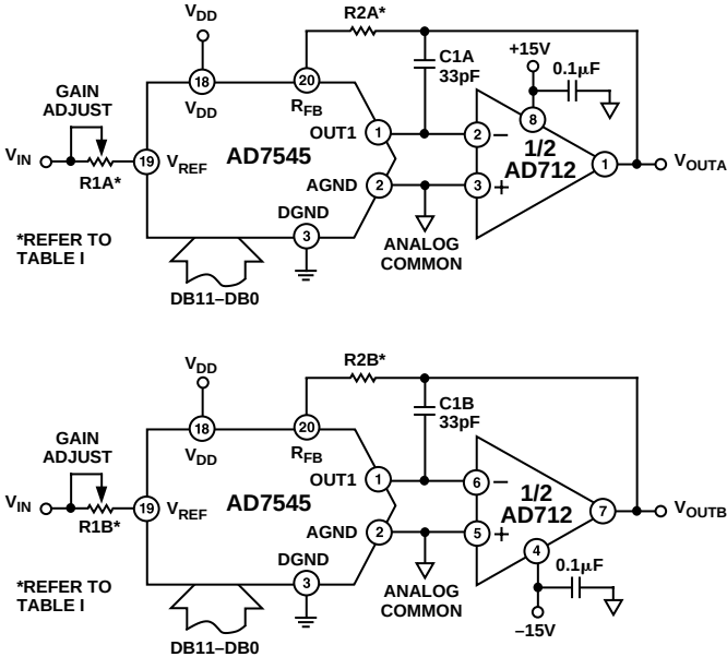
Figure 31. Unipolar Binary Operation
