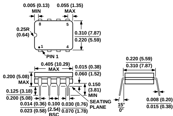
Cerdip (Q-8)
