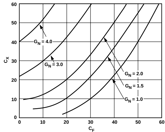
Figure 27. Value of Capacitor C_F vs. Value of C_X
