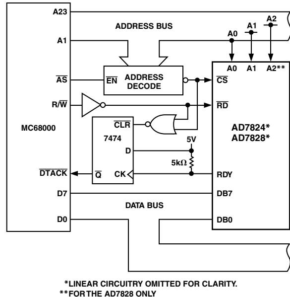
Figure 17. AD7824/AD7828–MC68000 Interface
