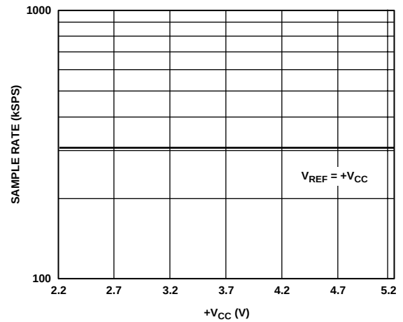
Figure 8. Maximum Sample Rate vs. +VCC
