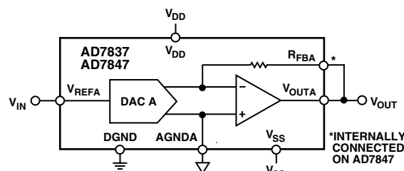
Figure 15. Unipolar Binary Operation
