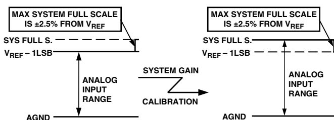
Figure 29. System Gain Calibration
