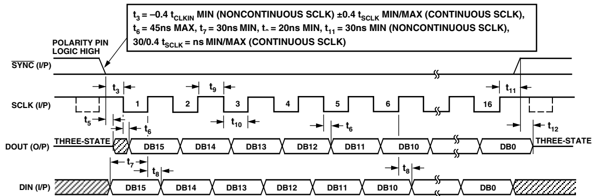
Figure 35. SPI/QSPI Mode 2 Timing Diagram for Read/Write Operation with \overline{\text{SYNC}} Input Edge Triggered ( \text{SM1} = \text{SM2} = 0 )
