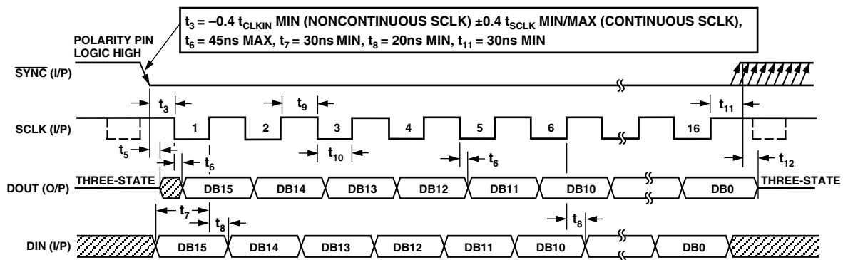
Figure 36. QSPI Mode 3 Timing Diagram for Read/Write Operation with \overline{\text{SYNC}} Input Edge Triggered ( \text{SM1} = 0 , \text{SM2} = 1 )
