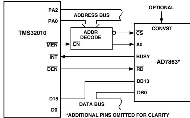
Figure 15. AD7863-TMS32010 Interface
