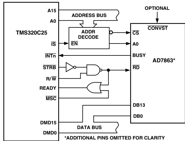
Figure 16. AD7863-TMS320C25 Interface
