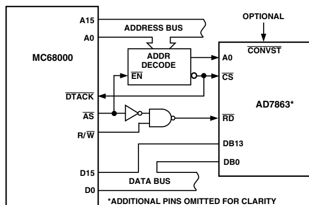
Figure 17. AD7863–MC68000 Interface
