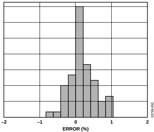
Figure 25. Typical Accuracy for Battery Channel ( 25^{\circ}\text{C} )
