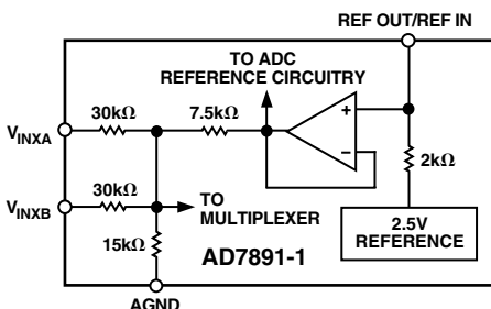
Figure 5. AD7891-1 Analog Input Structure
