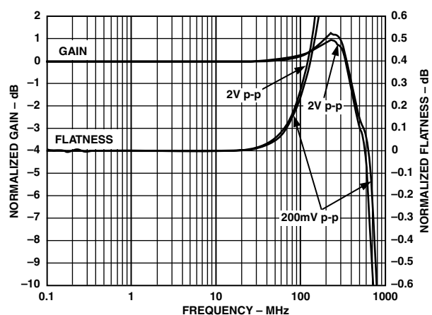
TPC 5. AD8075 Frequency Response; R_L = 1\ \text{k}\Omega , C_L = 5\ \text{pF}
