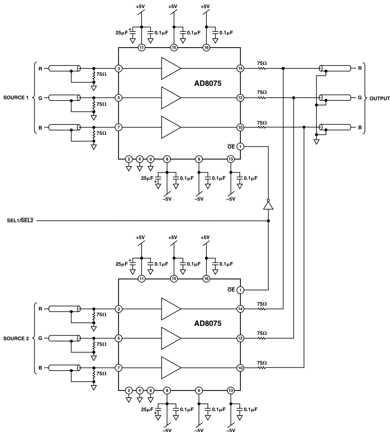
Figure 4. Mux
