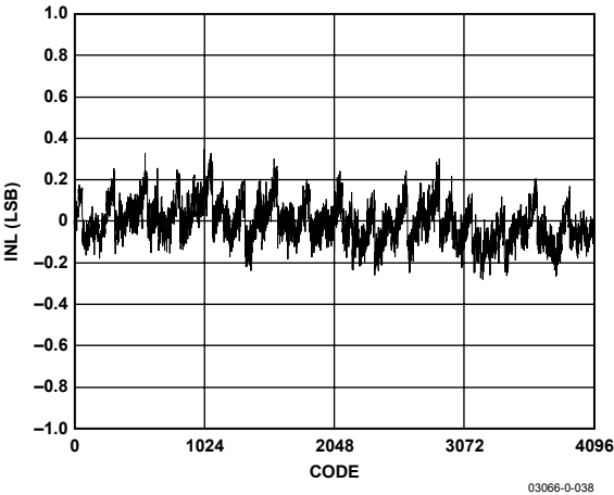
Figure 17. Typical INL
