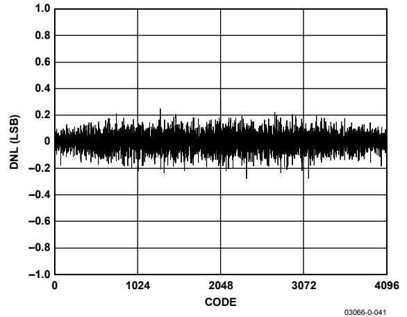
Figure 20. Typical DNL
