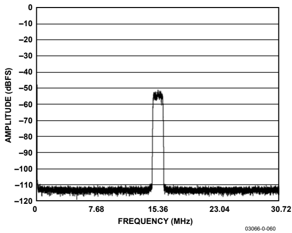
Figure 23. 32K FFT CDMA2K Carrier @ F_{IN} = 46.08 MHz: Sample Rate = 61.44 MSPS
