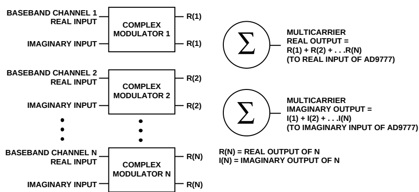
Figure 81. Synthesis of Multicarrier Complex Signal
