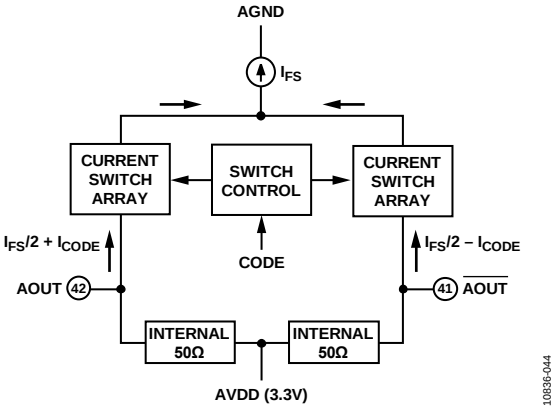
Figure 26. DAC Output
