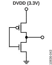
Figure 29. CMOS Output
