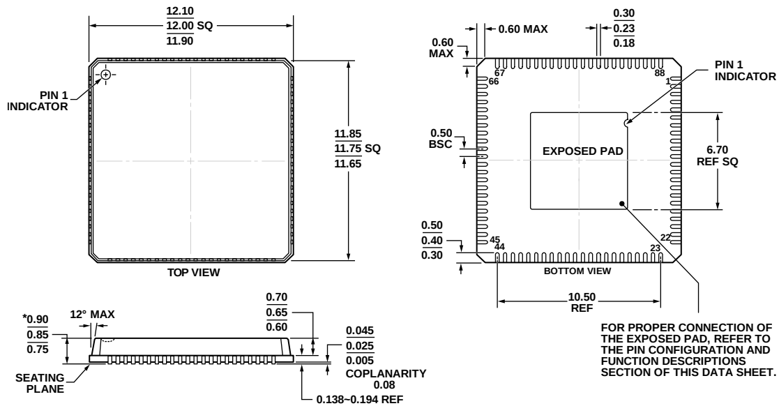
Figure 48. 88-Lead Lead Frame Chip Scale Package [LFCSP_VQ] 12 mm x 12 mm Body, Very Thin Quad (CP-88-5) Dimensions shown in millimeters
