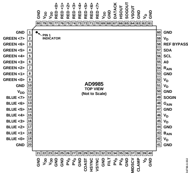
Figure 2. Pin Configuration
