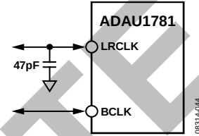
Figure 45. TDM Pulse Mode LRCLK Capacitor Alignment
