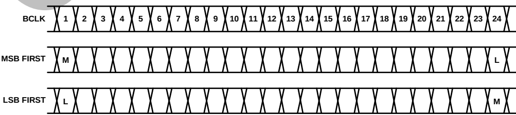
Figure 67. MSB Position Settings
