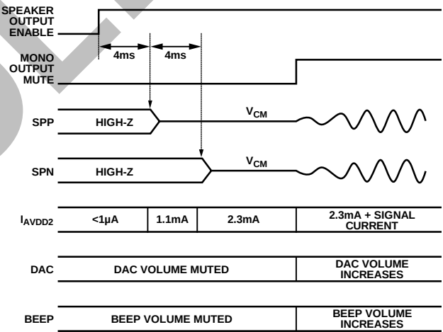
Figure 35. Speaker Driver Power-Up Sequence
