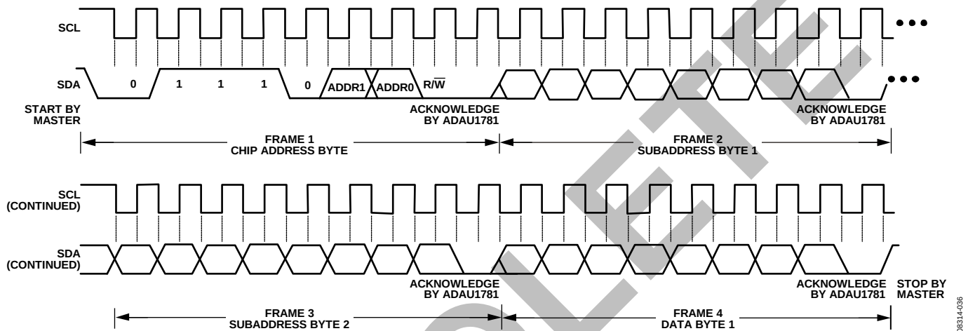
Figure 37. I²C Write to ADAU1781 Clcking
