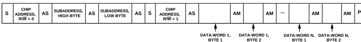
Figure 42. Burst Mode I 2 C Read Sequence
