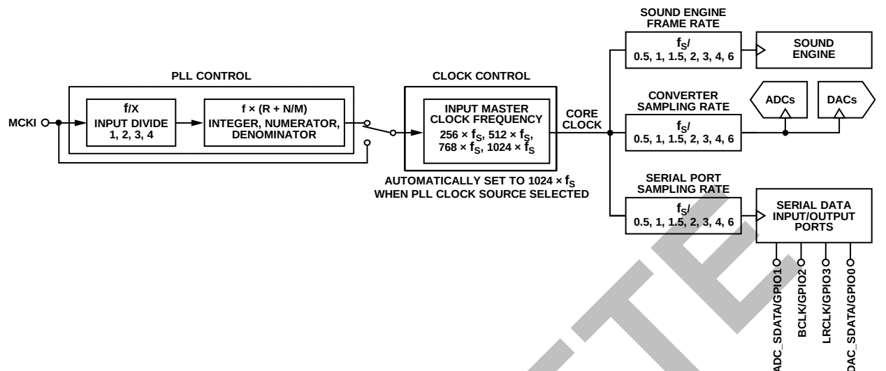
Figure 28. Clock Routing Diagram
