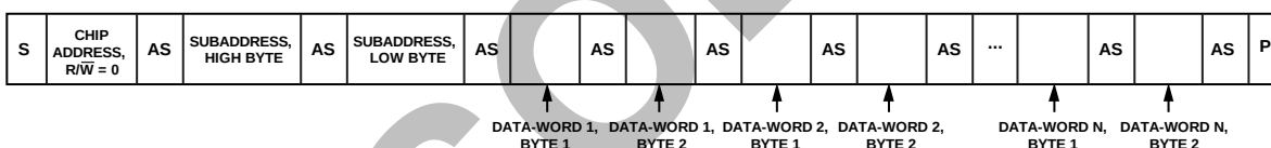
Figure 40. Burst Mode I 2 C Write Sequence
