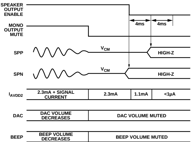
Figure 36. Speaker Driver Power-Down Sequence
