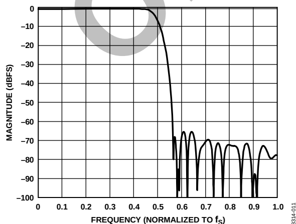
Figure 10. ADC Decimation Filter, 128x Oversampling, Normalized to f_s
