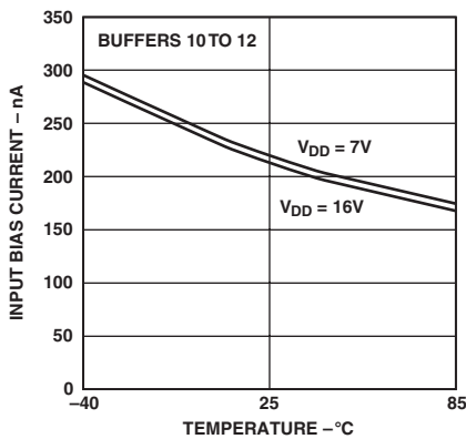
TPC 7. Input Bias Current vs. Temperature
