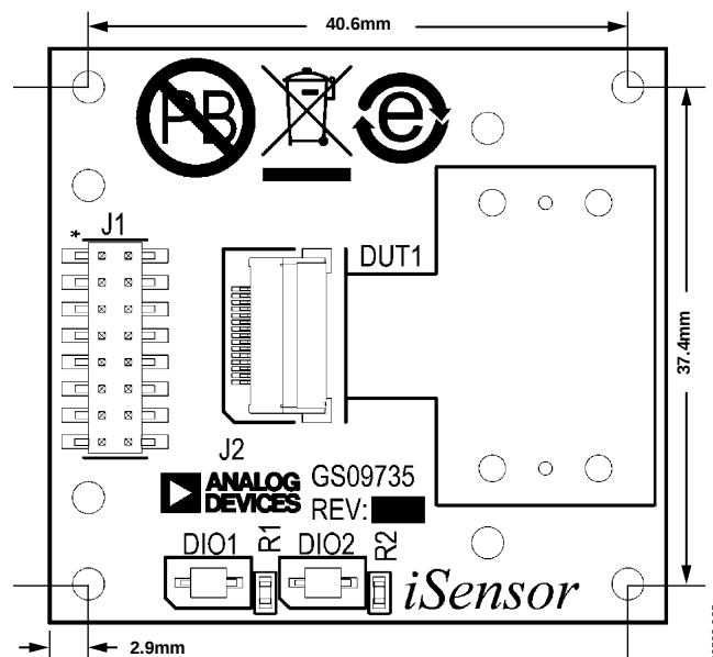
Figure 23. PCB Assembly View and Dimensions
