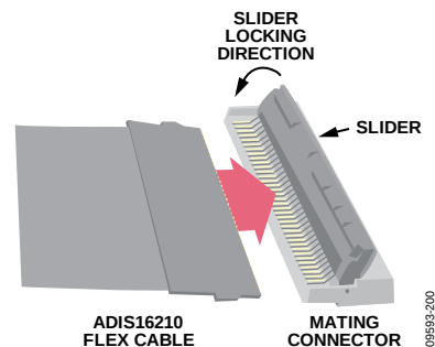
Figure 24. Mating Connector Detail
