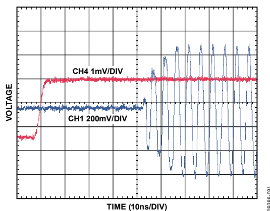
Figure 32. Enable Time Domain Response
