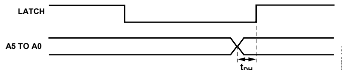
Figure 4. Parallel Mode Timing Diagram
