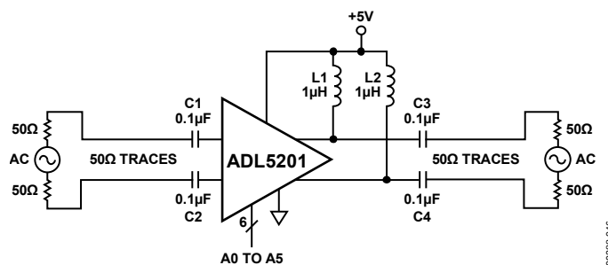
Figure 46. Test Circuit for S-Parameters on Dedicated 50 \Omega Differential-to-Differential Board
