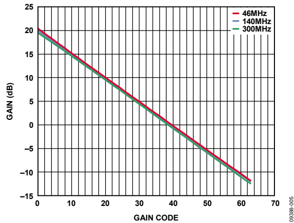
Figure 6. Gain vs. Gain Code at 46 MHz, 140 MHz, and 300 MHz
