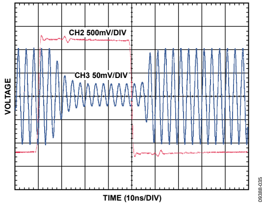
Figure 36. Gain Step Time Domain Response
