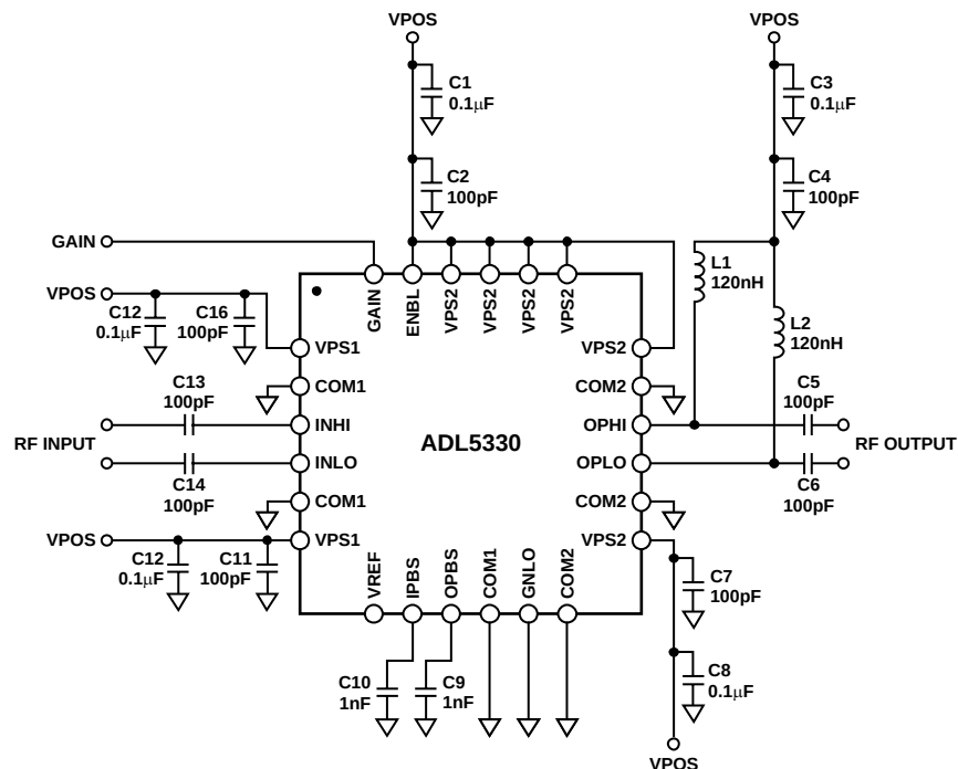
Figure 32. Basic Connections
