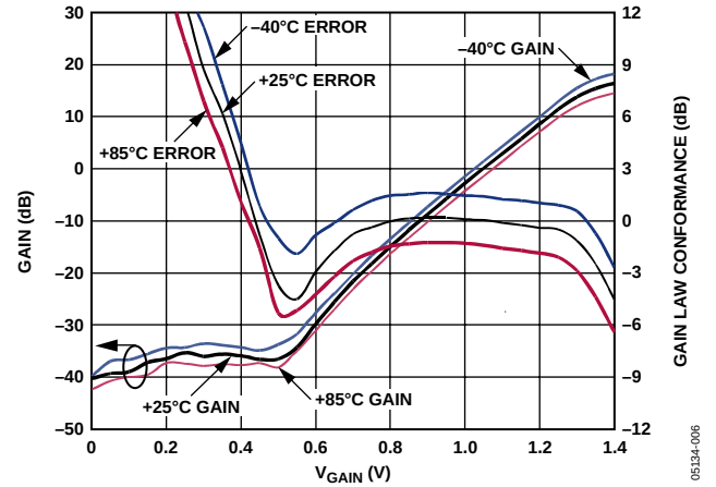
Figure 6. Gain and Gain Law Conformance vs. V_{\text{GAIN}} over Temperature at 2200 MHz
