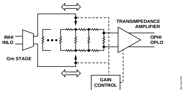
Figure 31. Simplified Schematic
