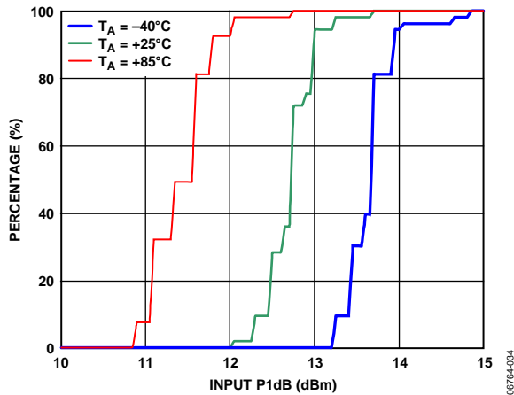
Figure 38. IP1dB Distributions
