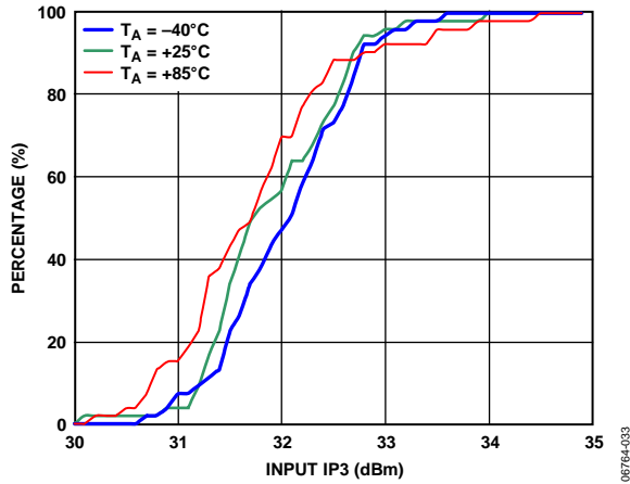
Figure 37. IIP3 Distributions
