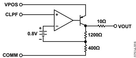
Figure 28. Output Interface
