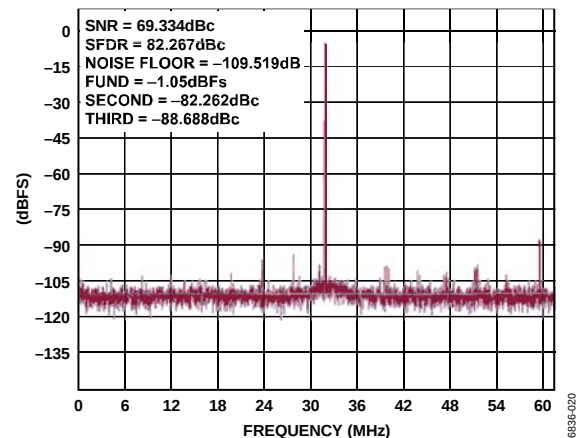
Figure 21. Measured Single-Tone Performance of the Circuit in Figure 19
