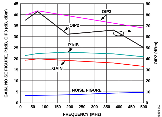
Figure 18. Performance of the ADL5534 Operating in Balanced Configuration
