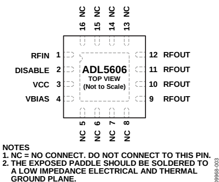
Figure 3. Pin Configuration
