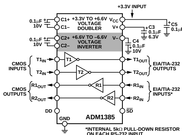
Figure 17. ADM1385 Typical Operating Circuit
